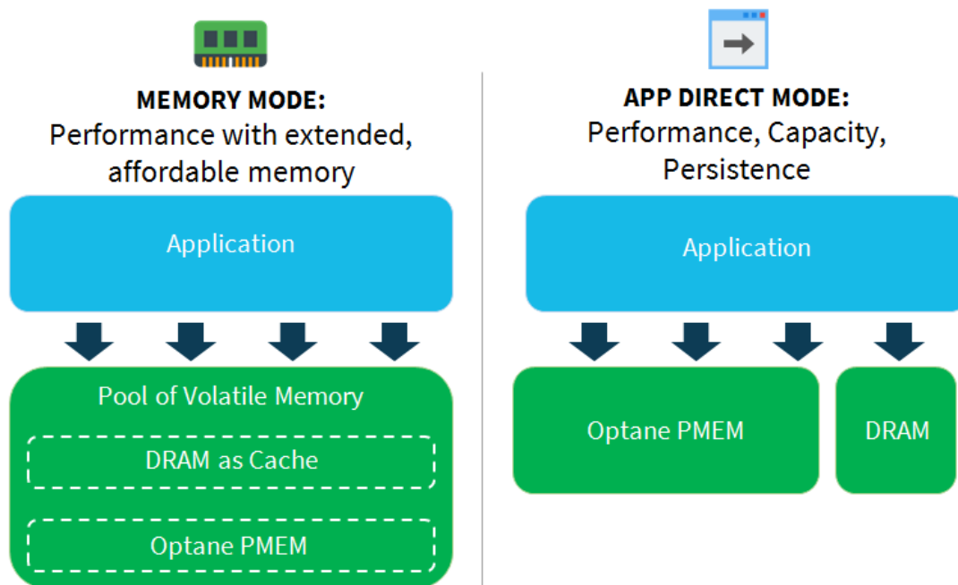
Figure 4. Intel Optane PMem: Memory Mode and App Direct Mode
