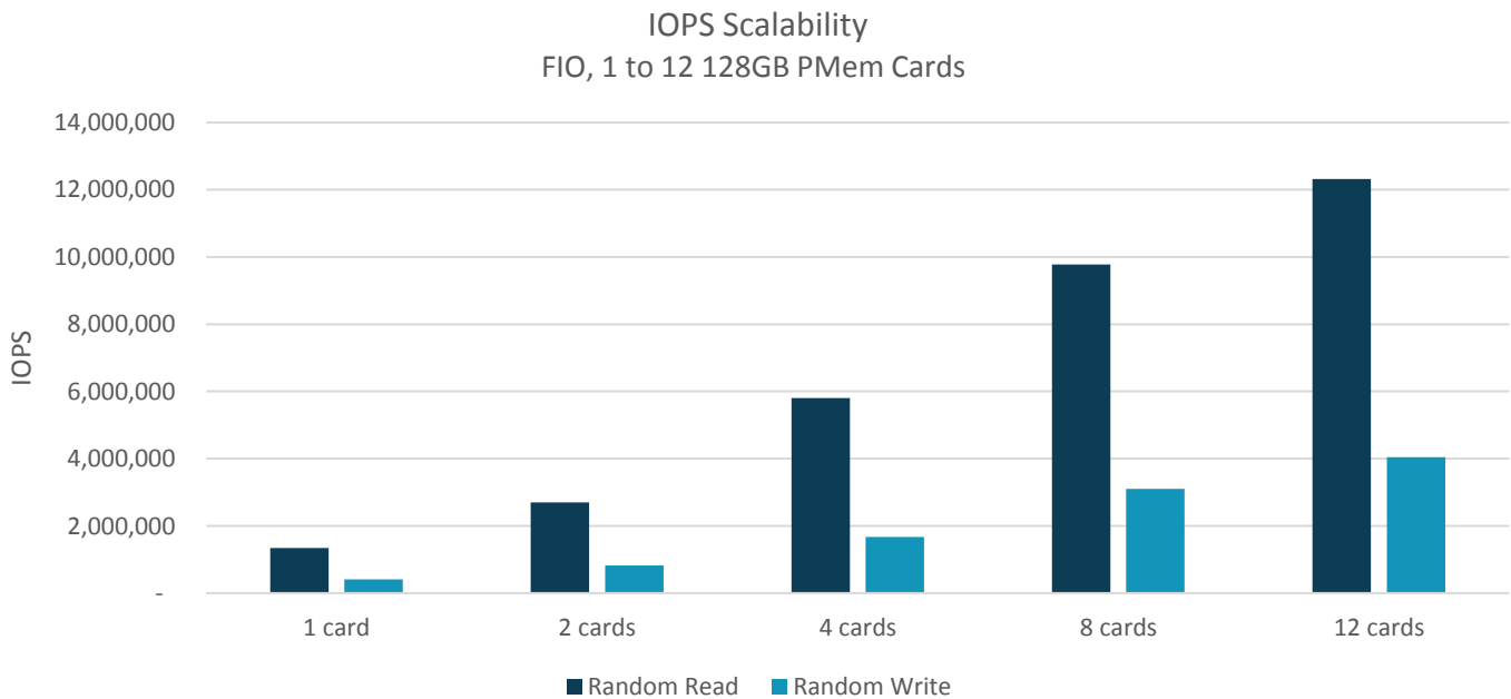
Figure 7. Near-linear IOPS Scalability
