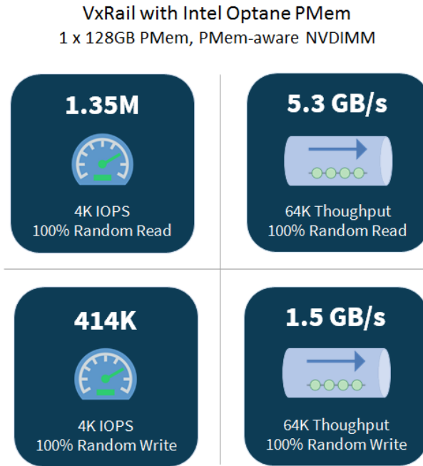
Figure 6. High-performance IOPS and Throughput, Single PMem Card
