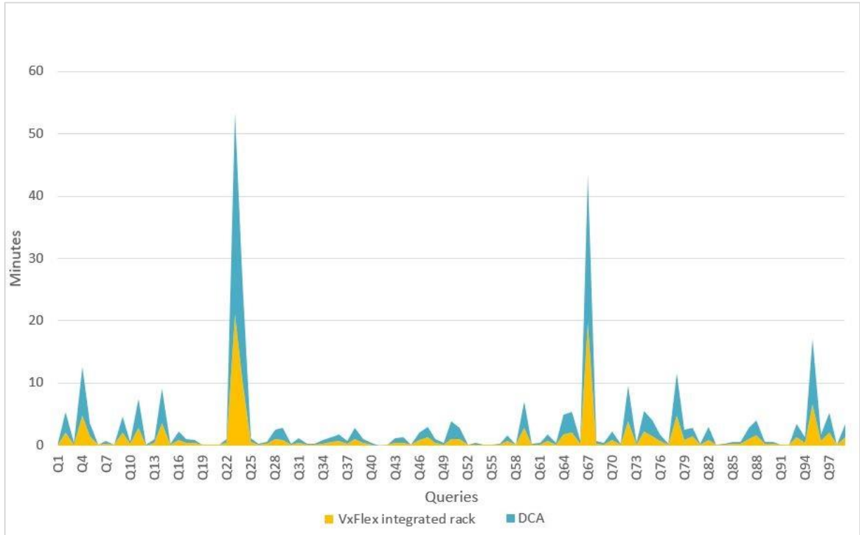
Figure 8 99 queries of VxFlex integrated rack vs. DCA
