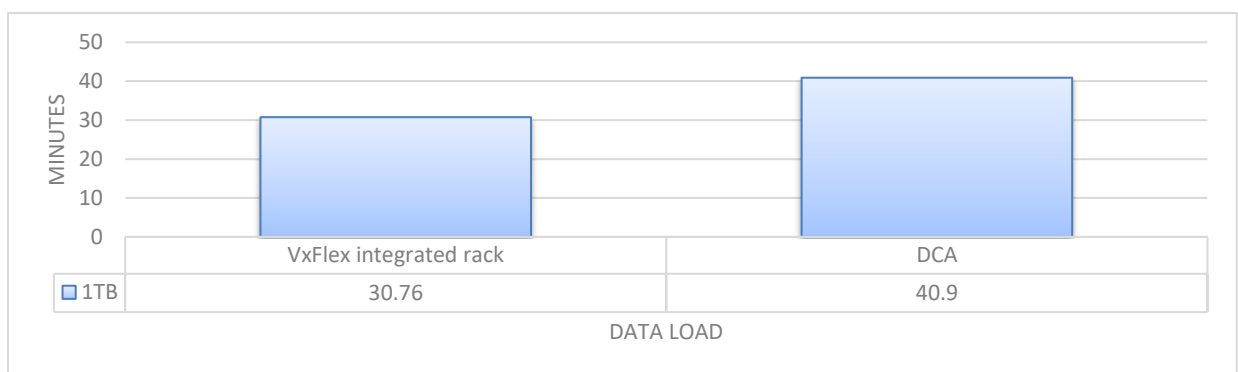
Figure 3 1 TB data load
