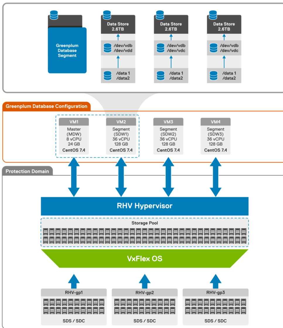
Figure 2 Pivotal Greenplum architecture diagram
