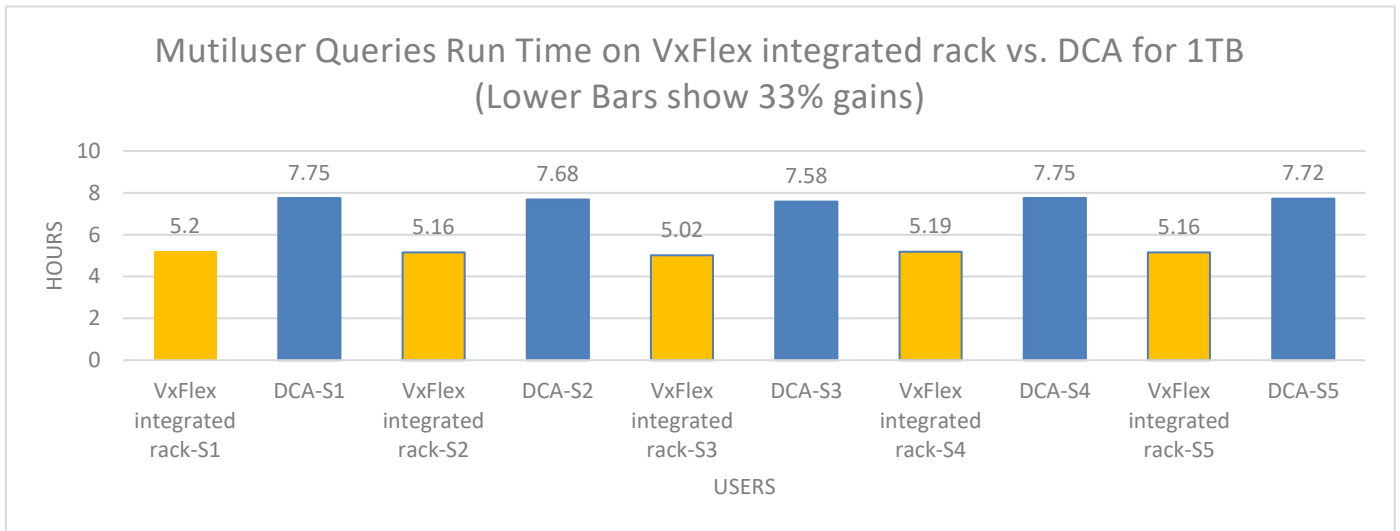
Figure 6 1 TB multiuser queries
