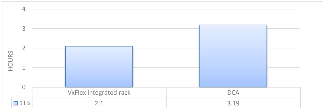
Figure 4 1 TB TPC-DS like single user total time query execution
