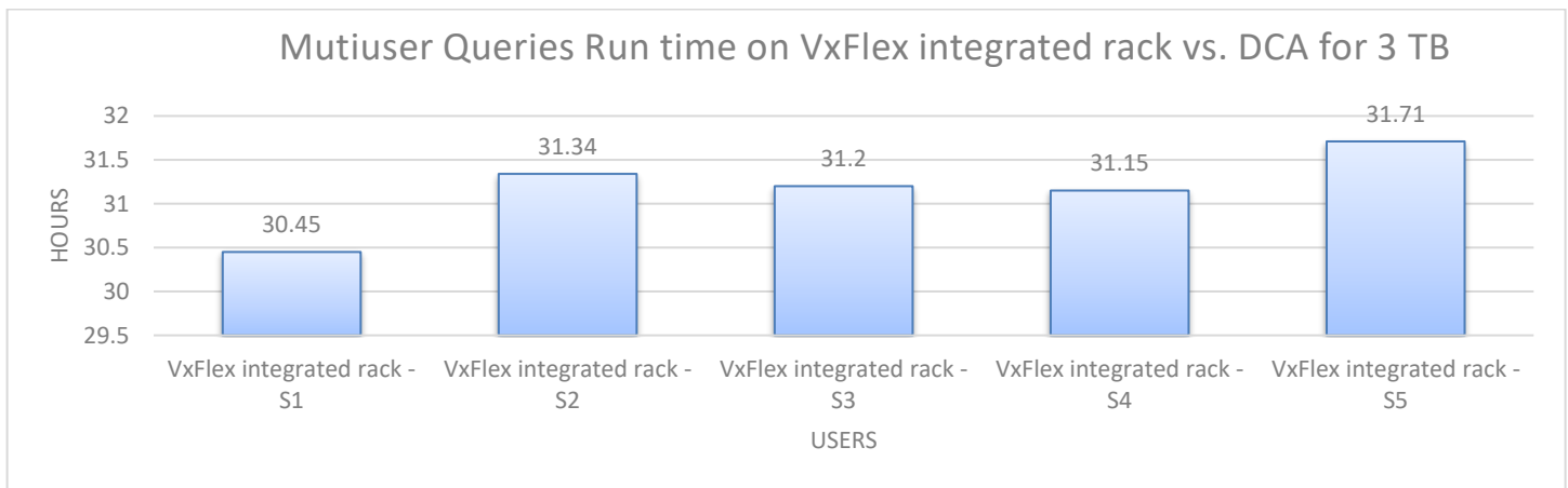
Figure 7 Multiuser queries run time on VxFlex integrated rack 3 TB
