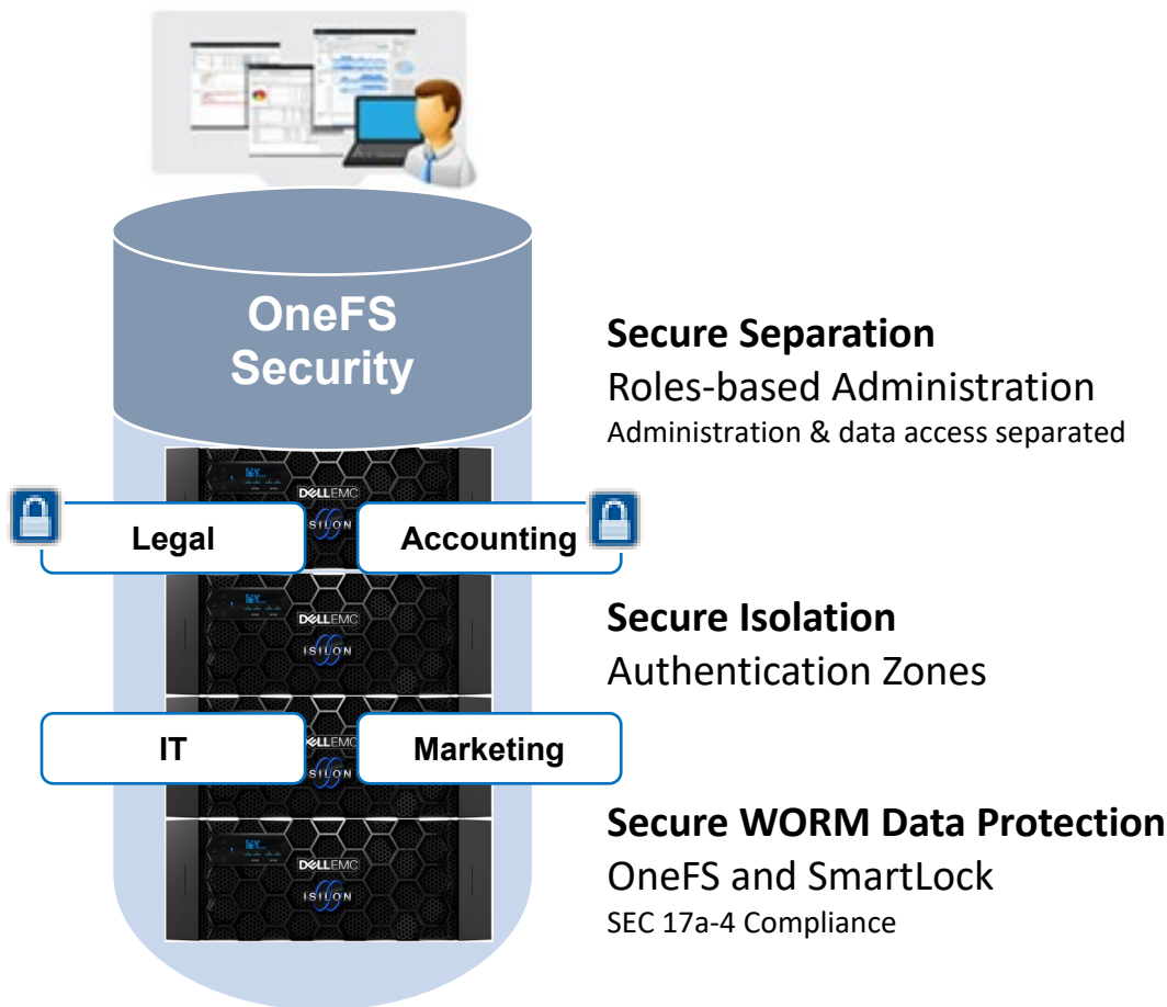
Figure 7: Isilon OneFS Security Options
