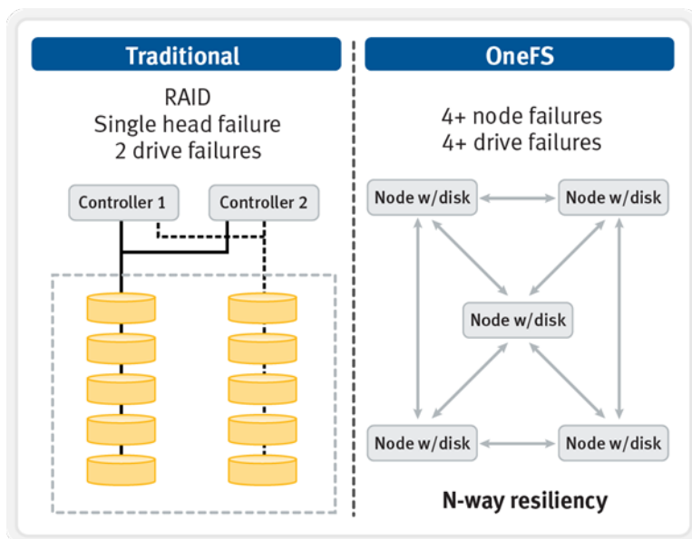
Figure 6: OneFS +4n Data Protection
