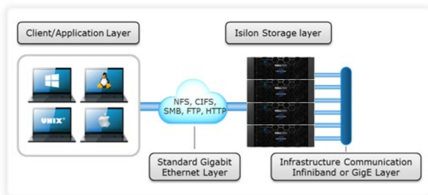
Figure 1: Isilon Scale-out NAS Architecture
