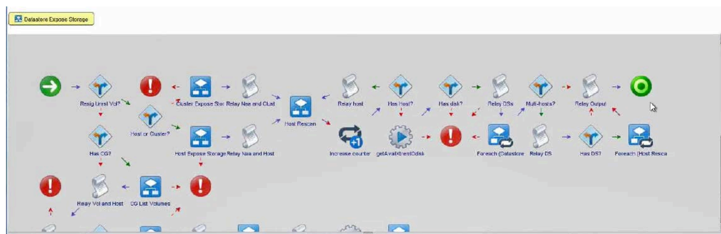
Figure 5. vRO Workflow
