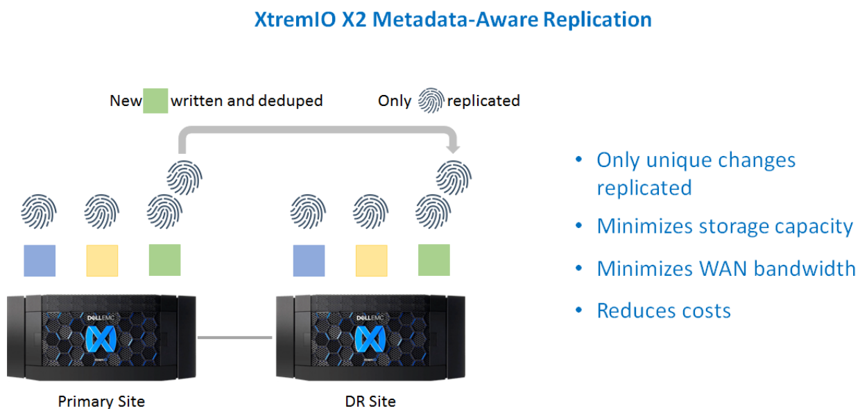
Figure 6. Metadata-Aware Replication
