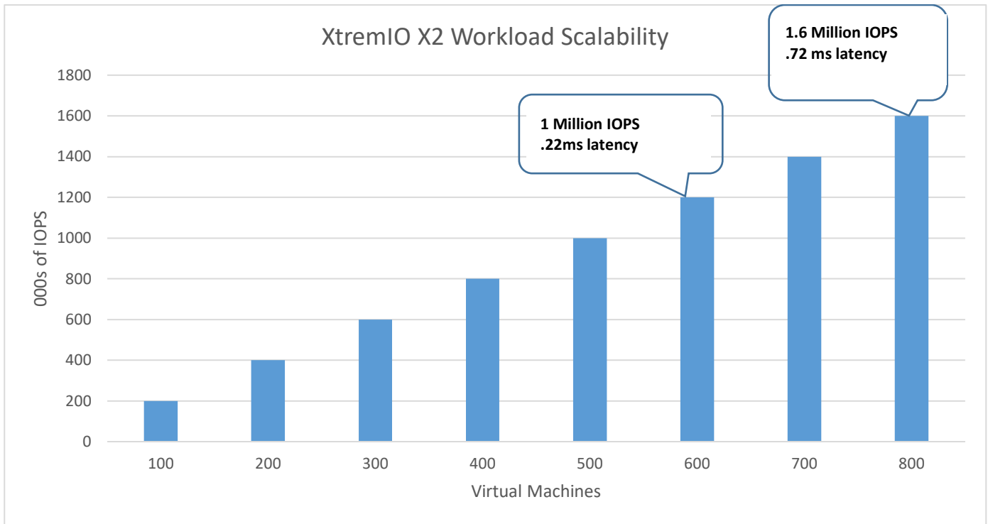
Figure 4. XtremIO X2 Workload Scalability: 800 VMs Created and Powered On
