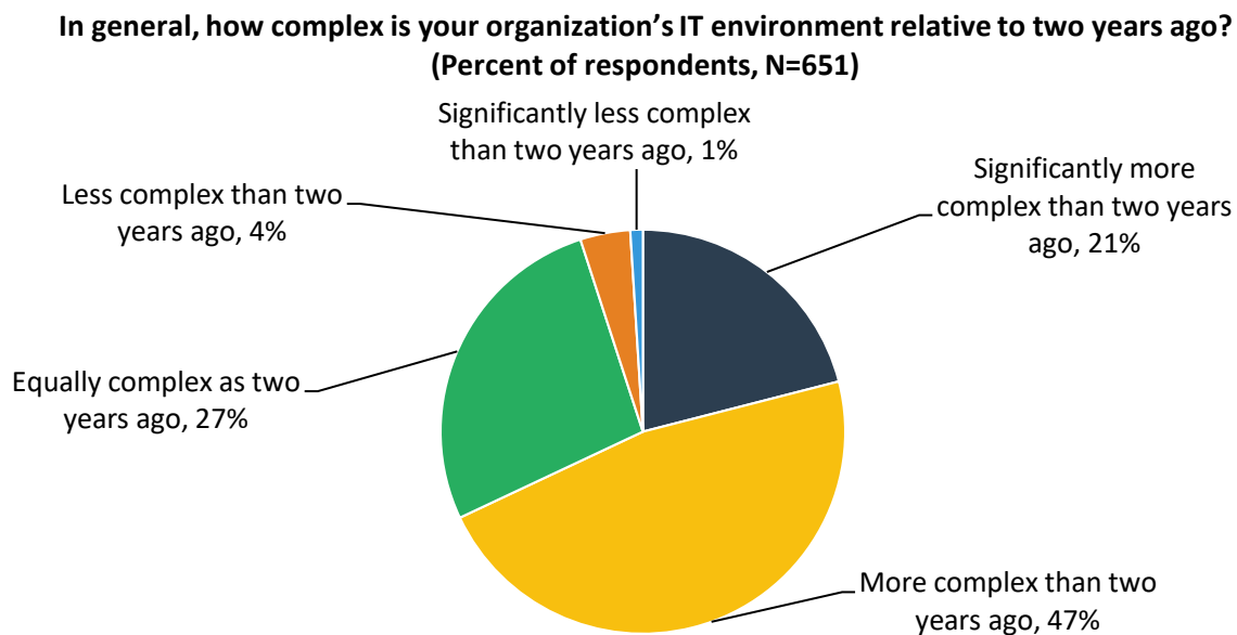
Figure 1. IT Complexity
