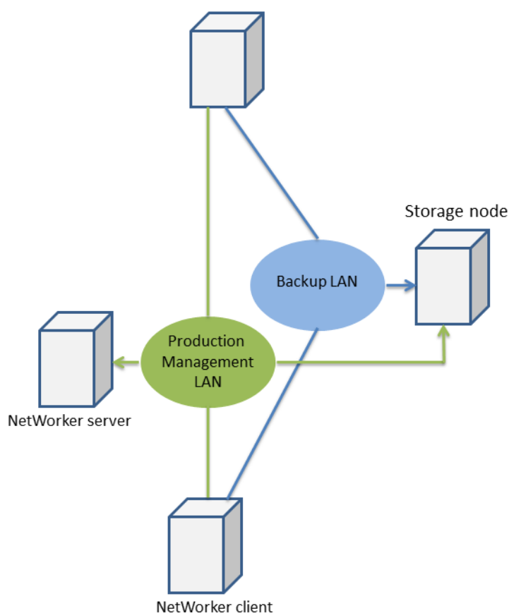
Figure 11 Sample network topology of NetWorker multihomed backup
