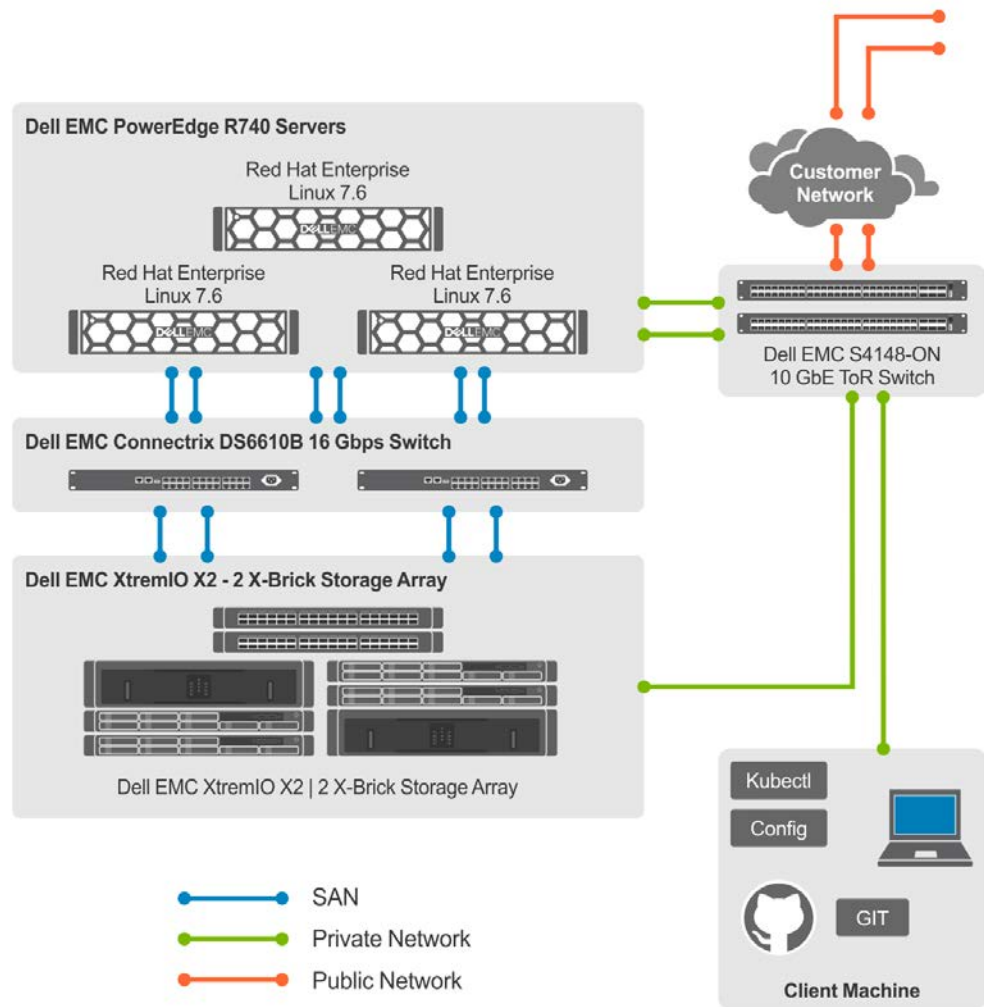
Figure 18. Solution architecture
