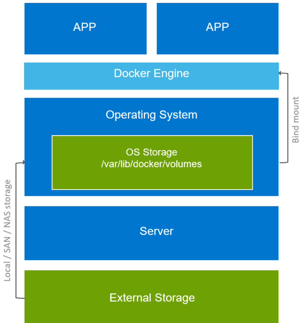
Figure 4. Bind mount
